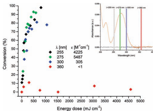
Figure 3. Conversion (%) of the photocleavage at the surface of the chromophore pHP-CPTS upon irradiation at different wavelengths and the UV spectrum of the corresponding silane (inset).
